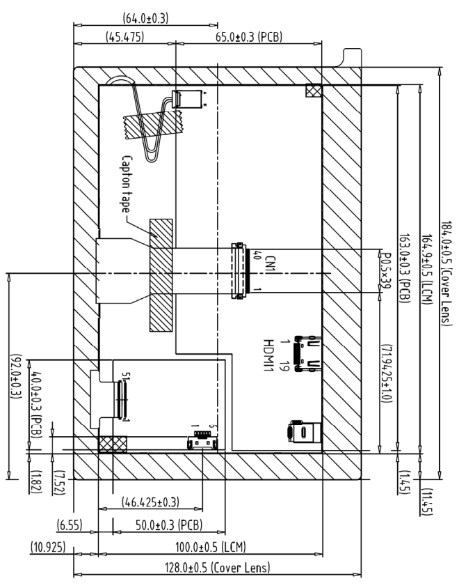
Back View
